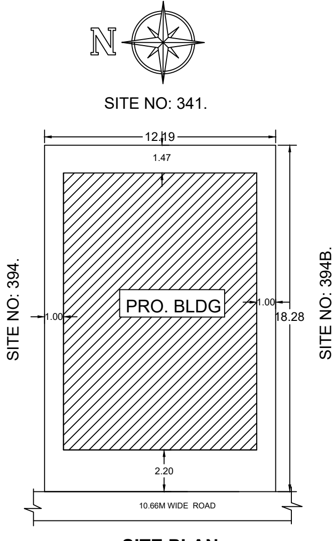
SITE PLAN
